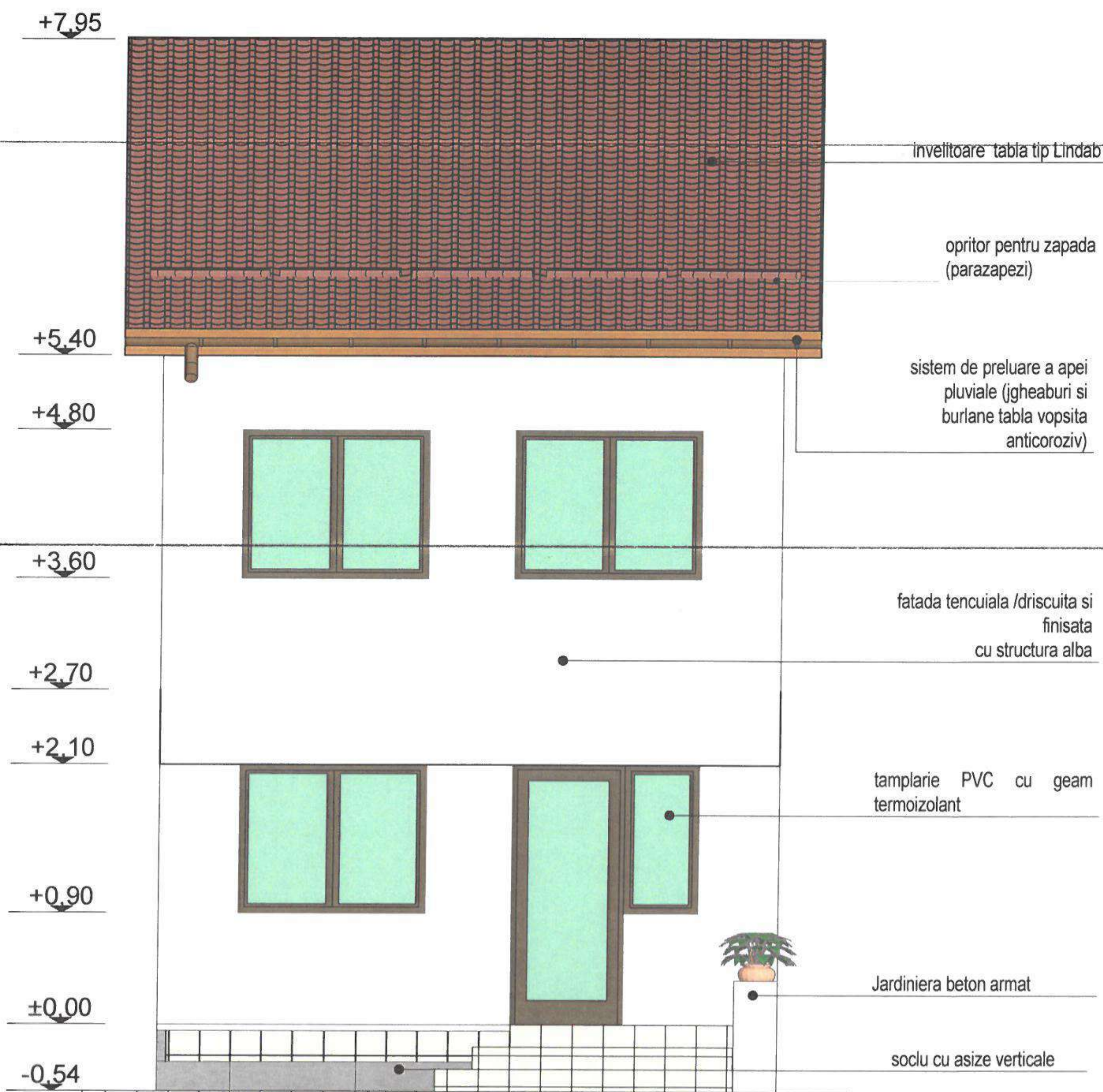
FATADA PRINCIPALA SC 1/50
