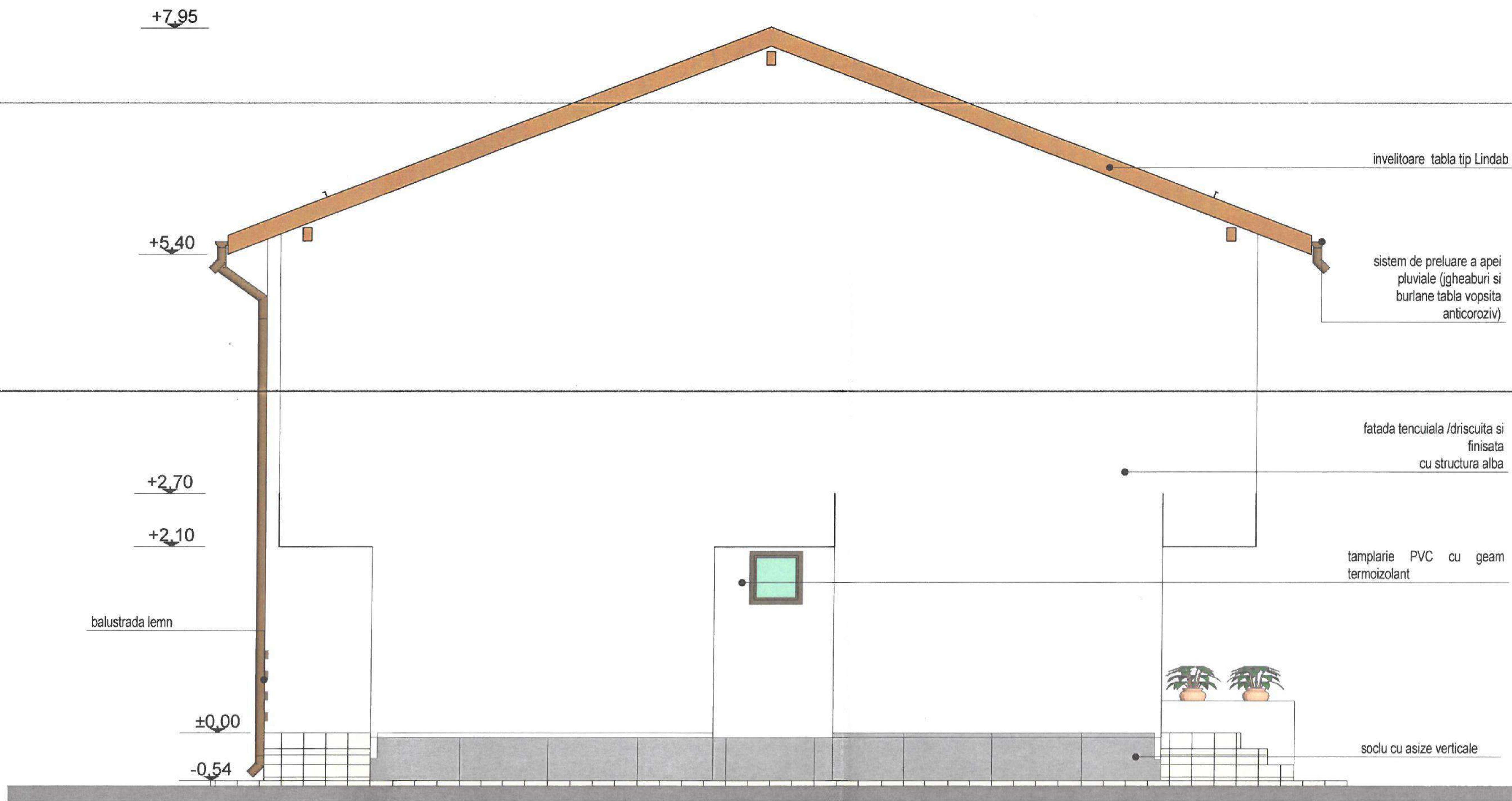
FATADA LATERALA STANGA SC 1/50
