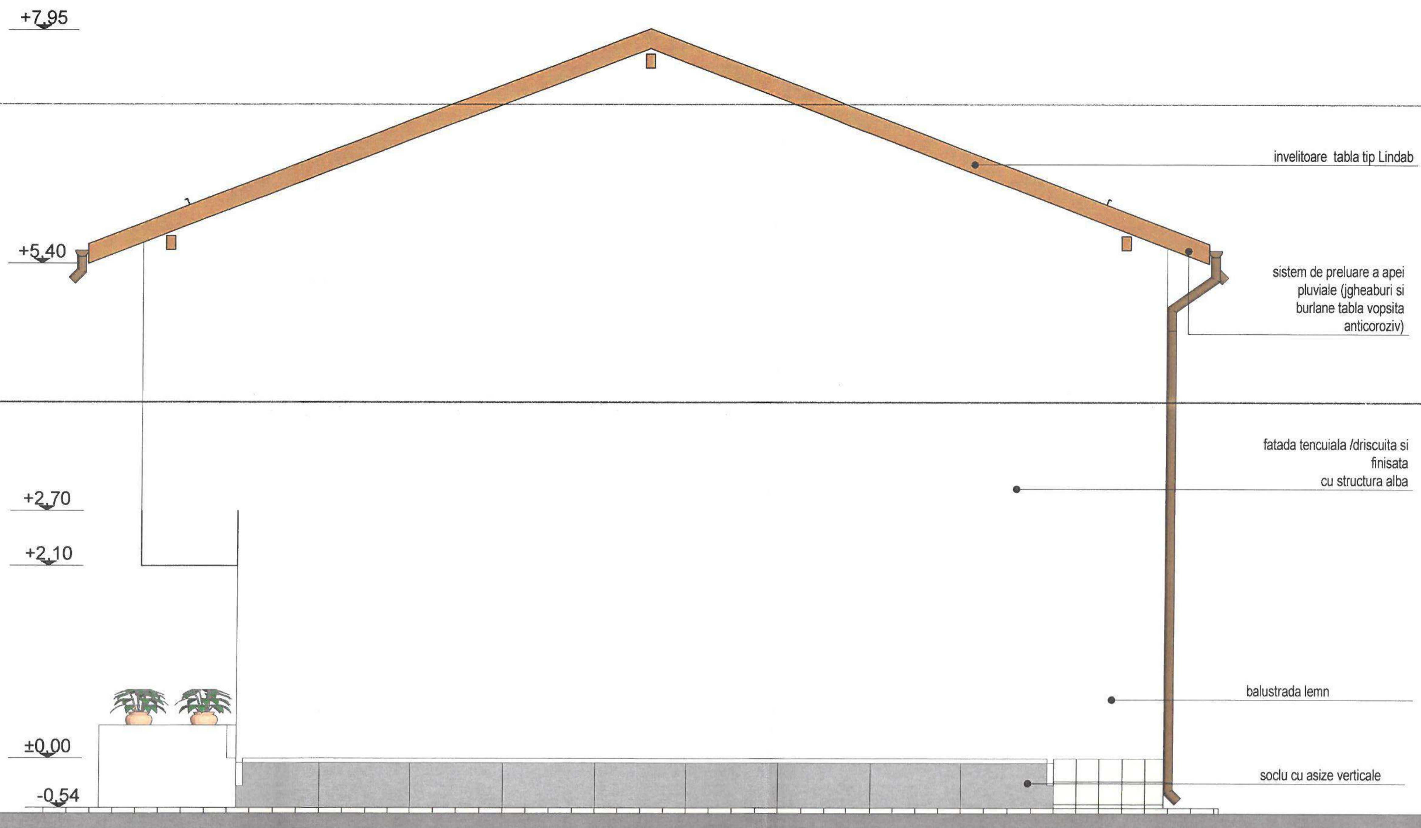
FATADA LATERALA DREAPTA SC 1/50
